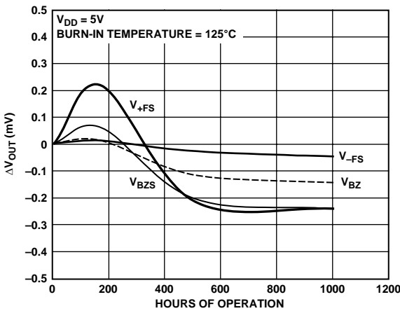
Figure 14. Long-Term Drift
